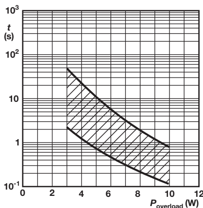
NFR25 This graph is based on measured data which may deviate according to the application. Fusing Characteristics: 15 \Omega \leq R \leq 15 \text{ k}\Omega
