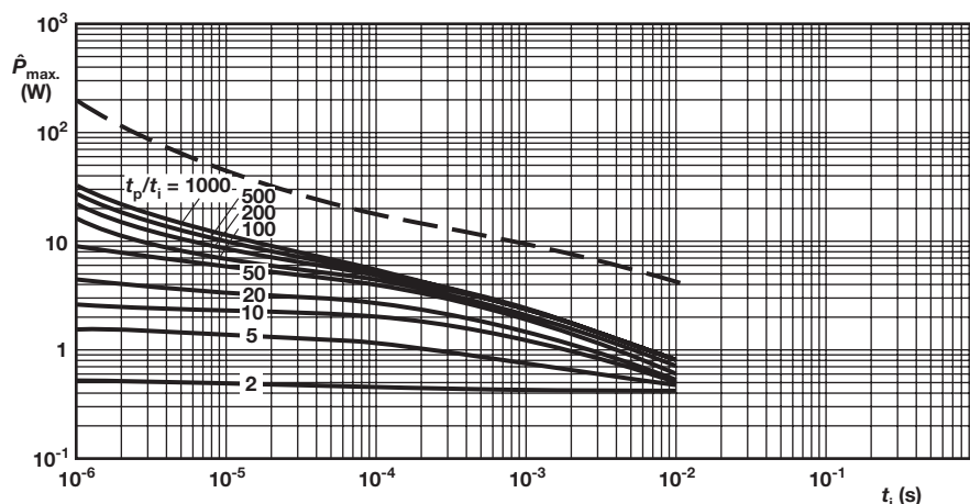
NFR25 Pulse on a regular basis; maximum permissible peak pulse power ( \hat{P}_{\max.} ) as a function of pulse duration ( t_i ), 0.22 \Omega \leq R \leq 15 \text{ k}\Omega
