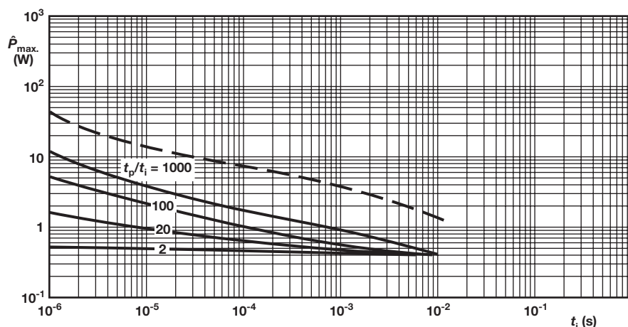
NFR25 Pulse on a regular basis; maximum permissible peak pulse power ( \hat{P}_{\max.} ) as a function of pulse duration ( t_i ), 15 \text{ k}\Omega \leq R \leq 15 \text{ k}\Omega
