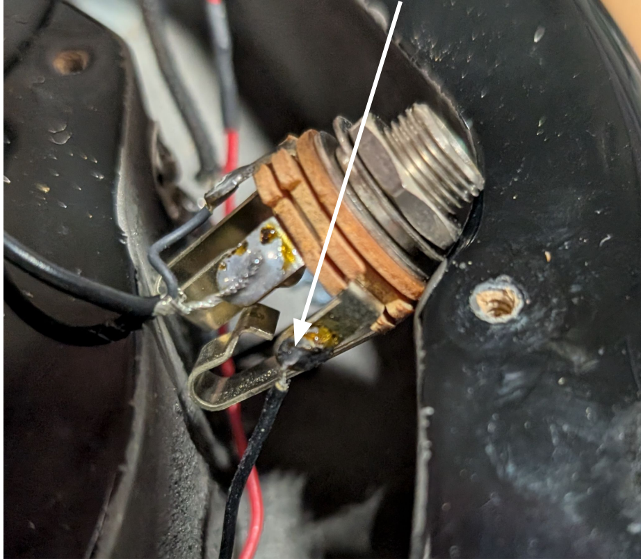
Battery -ve
