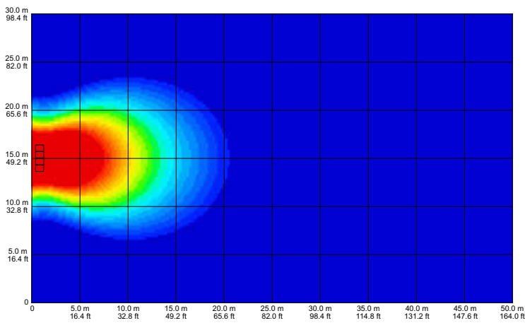
fig 5. four vertically positioned enclosures horizontally arrayed 100Hz
