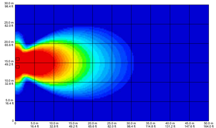
fig 40. two vertically positioned enclosures 2 m (6.6 ft) spacing 100Hz
