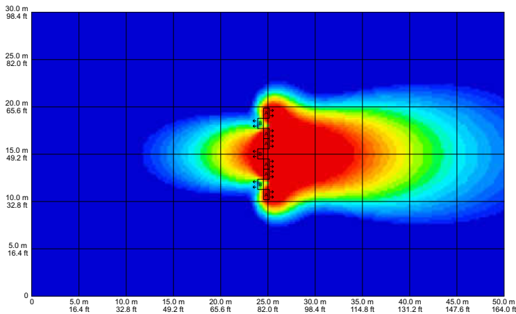
fig 90. four enclosure high Delta Array 50Hz
