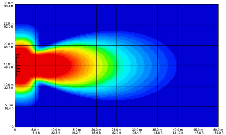
fig 15. eight vertically positioned enclosures horizontally arrayed 100Hz
