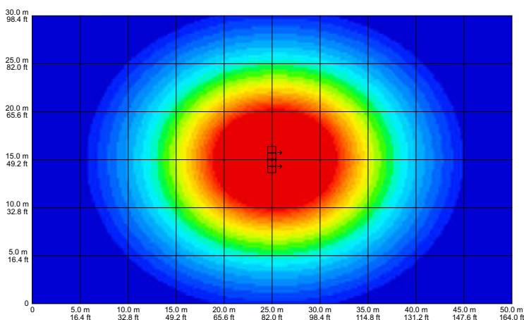
fig 7. four vertically positioned enclosures horizontally arrayed 50Hz
