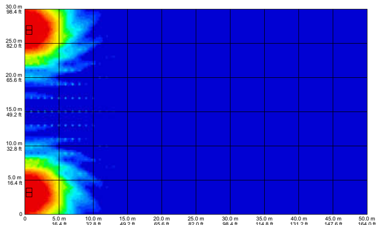
fig 54. two groups of two vertically positioned enclosures 24 m (78.7 ft) spacing 50Hz
