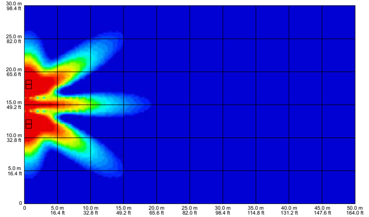
fig 50. two groups of two vertically positioned enclosures 6 m (19.7 ft) spacing 100Hz
