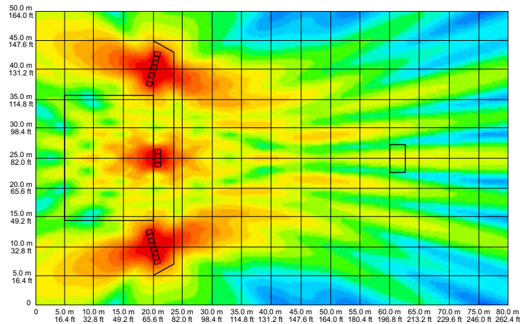
fig 127. two groups of eight vertically positioned enclosures 15 degree toe in with 4 vertically positioned centre enclosures delayed by 36 ms 100Hz
