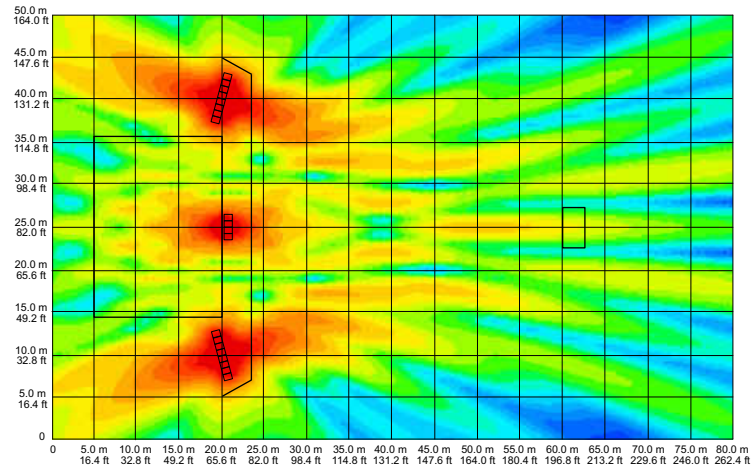
fig 125. two groups of eight vertically positioned enclosures 15 degree toe in with 4 vertically positioned centre enclosures not delayed 100Hz
