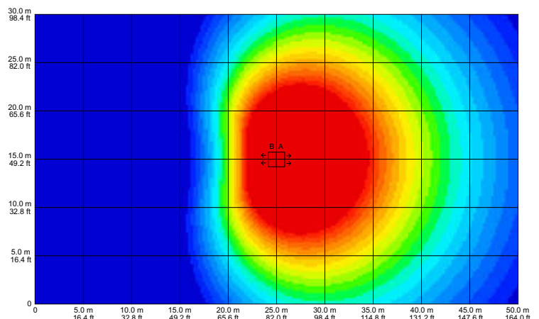
fig 78. two horizontally positioned enclosures back to back enclosure B phase reversed with 3 ms delay 100Hz
