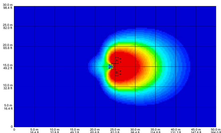
fig 80. two enclosure high Delta Array 50Hz
