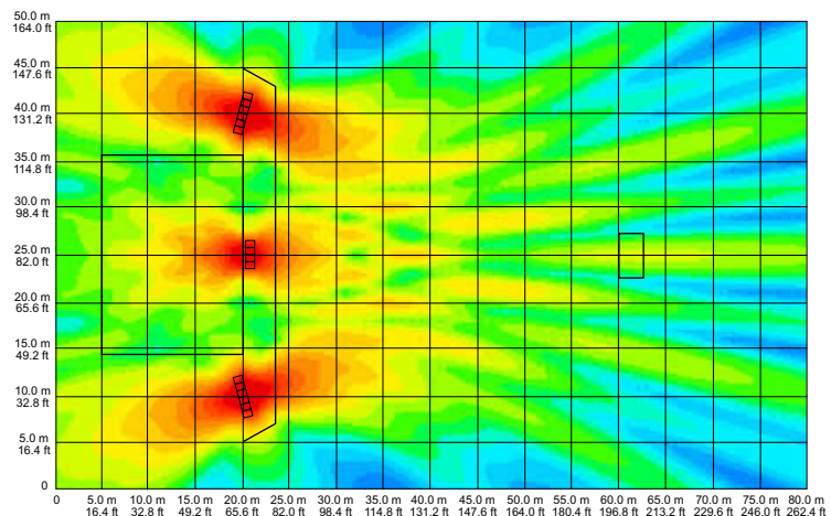
fig 117. two groups of six vertically positioned enclosures 15 degree toe in with 4 vertically positioned centre enclosures delayed by 36 ms 100Hz
