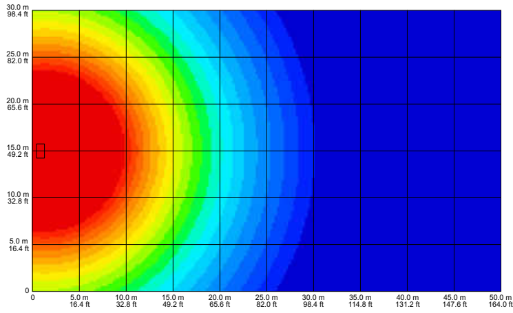
fig 35. eight horizontally positioned enclosures vertically arrayed 100Hz
