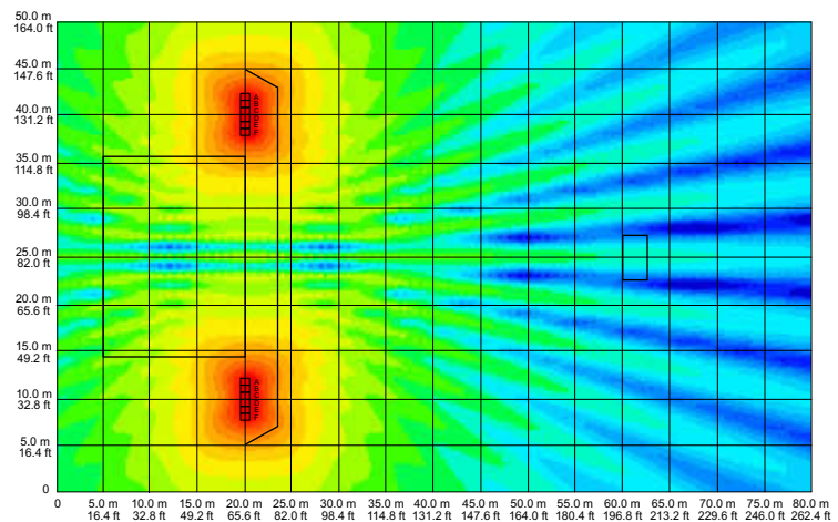
fig 105. two groups of six vertically positioned enclosures 3.6 ms delay applied to enclosures A and F 100Hz
