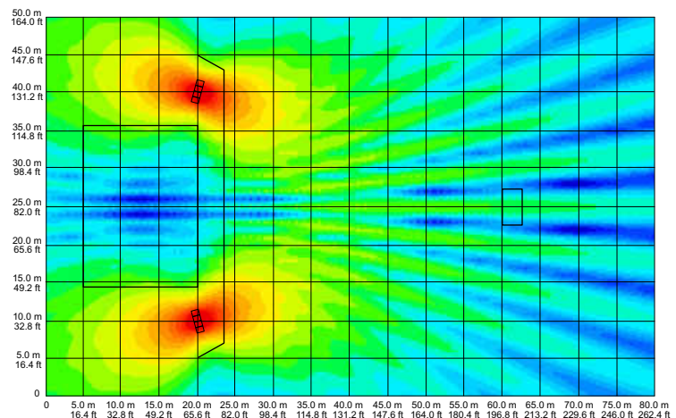
fig 99. two groups of four vertically positioned enclosures 15 degree toe in 100Hz
