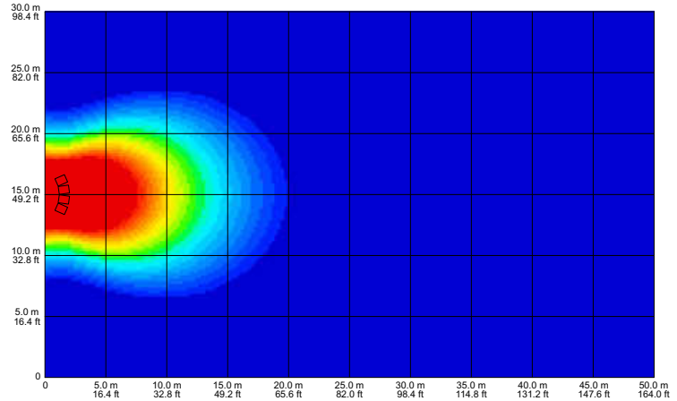
fig 20. four vertically positioned enclosures horizontally arrayed 100Hz 12 degree spacing between enclosures forming a curve
