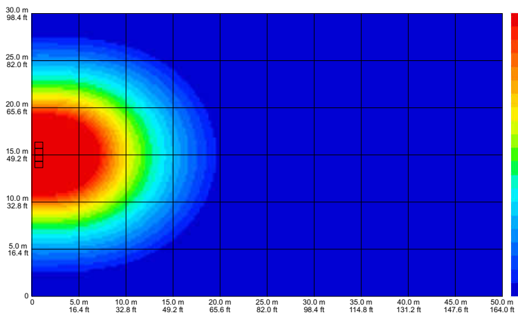
fig 4. four vertically positioned enclosures horizontally arrayed 50Hz
