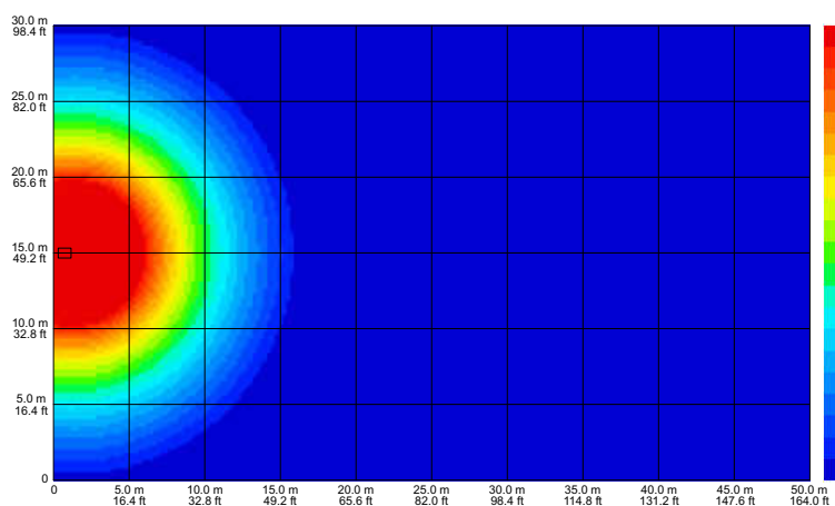
fig 1. single vertically positioned enclosure 50Hz
