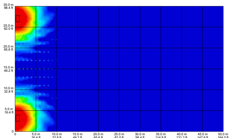
fig 66. two groups of two horizontally positioned enclosures vertically arrayed with a 24 m (78.7 ft) spacing 50Hz
