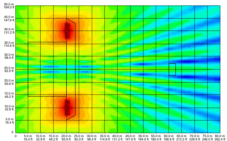
fig 121. two groups of eight vertically positioned enclosures 100Hz 3.6 ms delay applied to A and H, 1.1 ms delay applied to B and G
