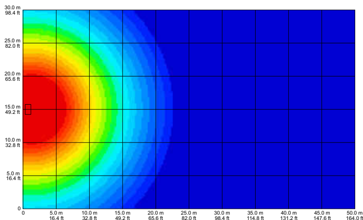
fig 13. six horizontally positioned enclosures vertically arrayed 100Hz
