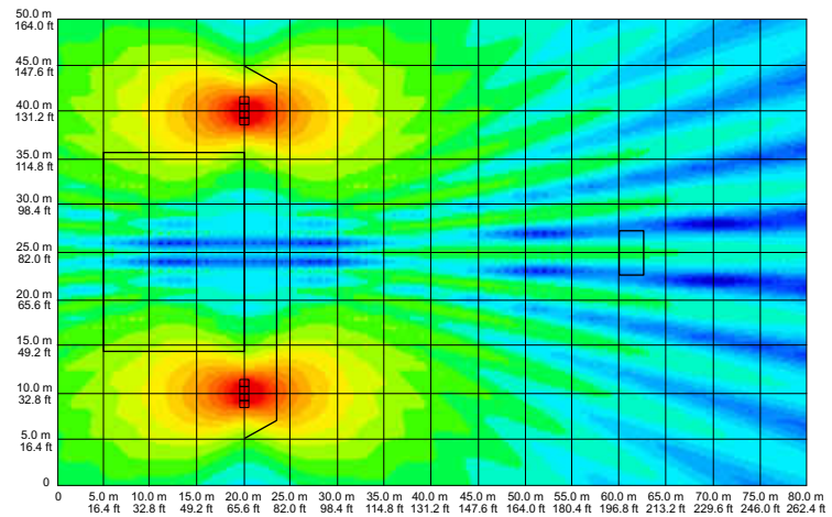
fig 97. two groups of four vertically positioned enclosures 100Hz
