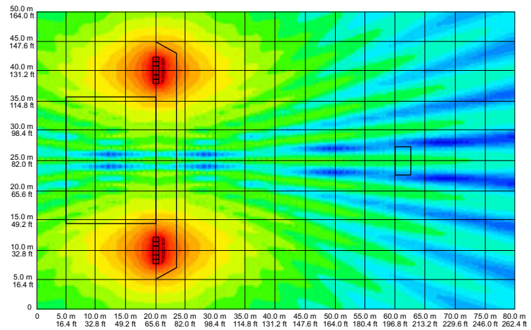
fig 103. two groups of six vertically positioned enclosures 2.4 ms delay applied to enclosures A and F 100Hz
