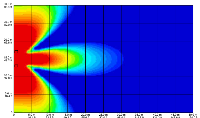
fig 42. two vertically positioned enclosures 4 m (13.1 ft) spacing 100Hz
