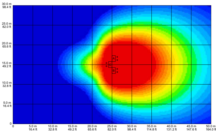
fig 85. four enclosure high Delta Array 50Hz
