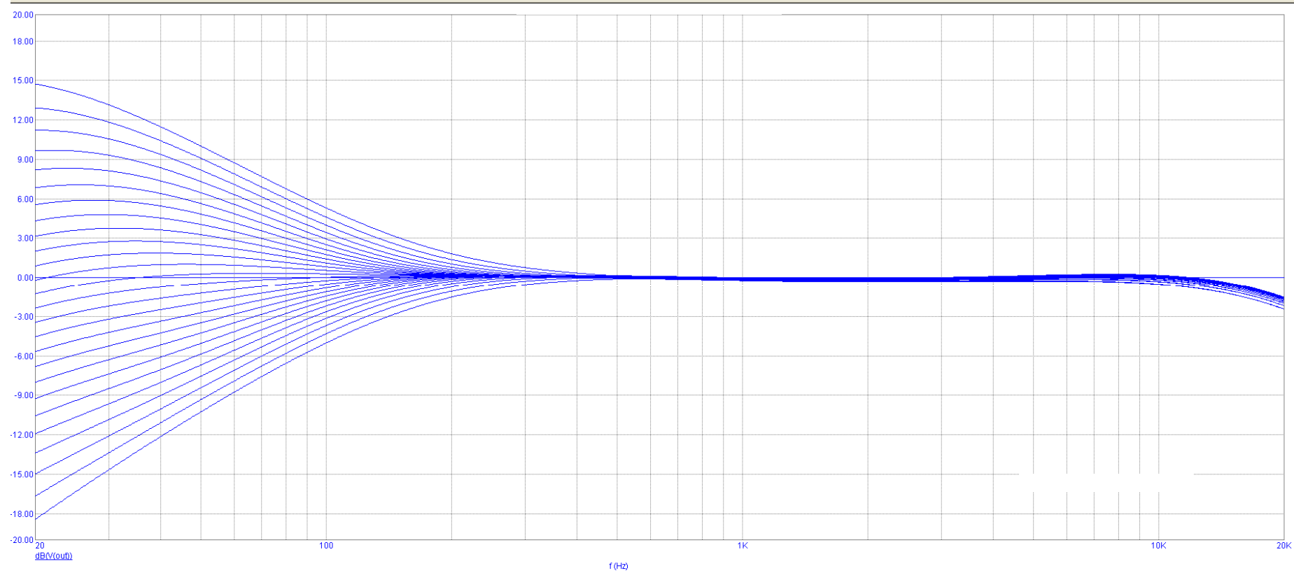
Frequency response – low control min/max
