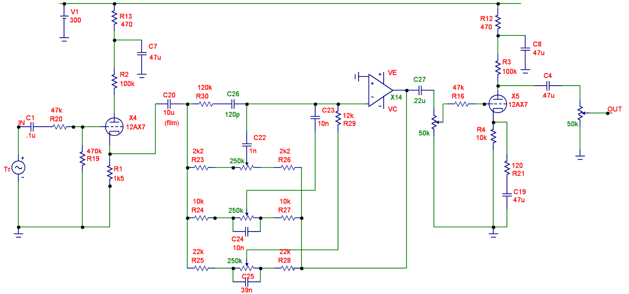
Bass preamp schematic diagram V1.0
