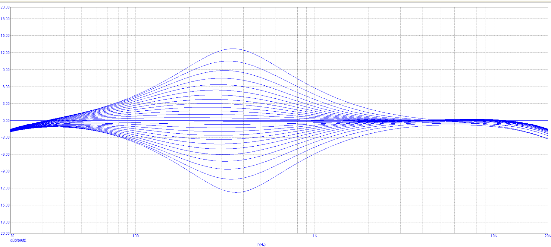
Frequency response – mid control min/max ; C24 = 10nF
