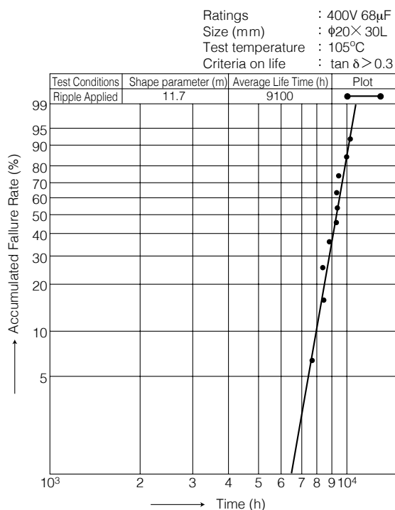
Fig. 2-12 Failure Analysis by Weibull Probability Paper
