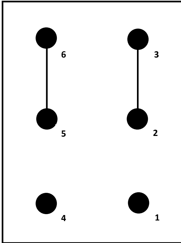
DPDT ON-ON-ON, position 1
