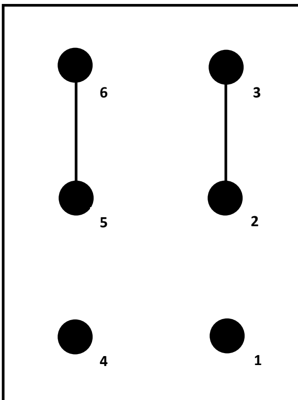
DPDT ON-ON, position 1
