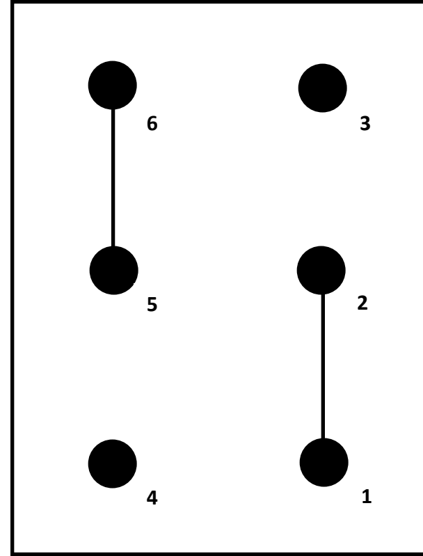
DPDT ON-ON-ON, position 2
