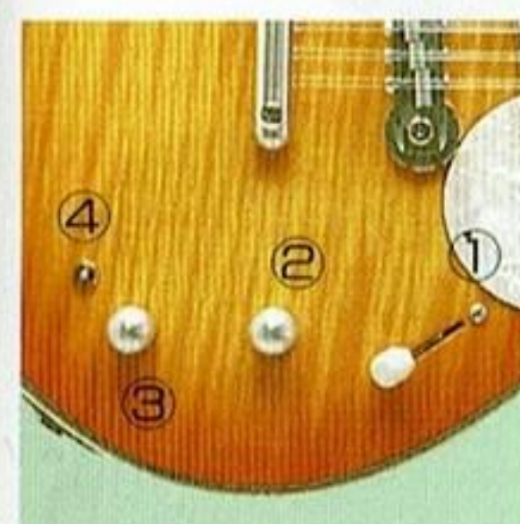
(TGX-823/812 Controls) 1. Pickup selector switch 2. Master volume 3. Master tone 4. 3way selector switch (Active 1, passive, Active 2)
