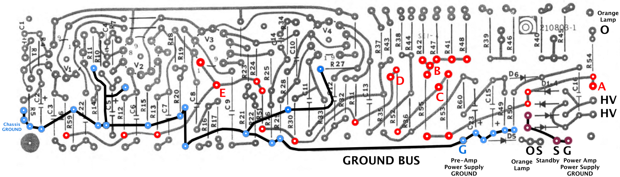
V4B Main Printed Circuit Board Copper Side
