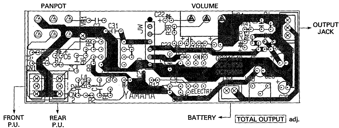
Components side (部品側)
